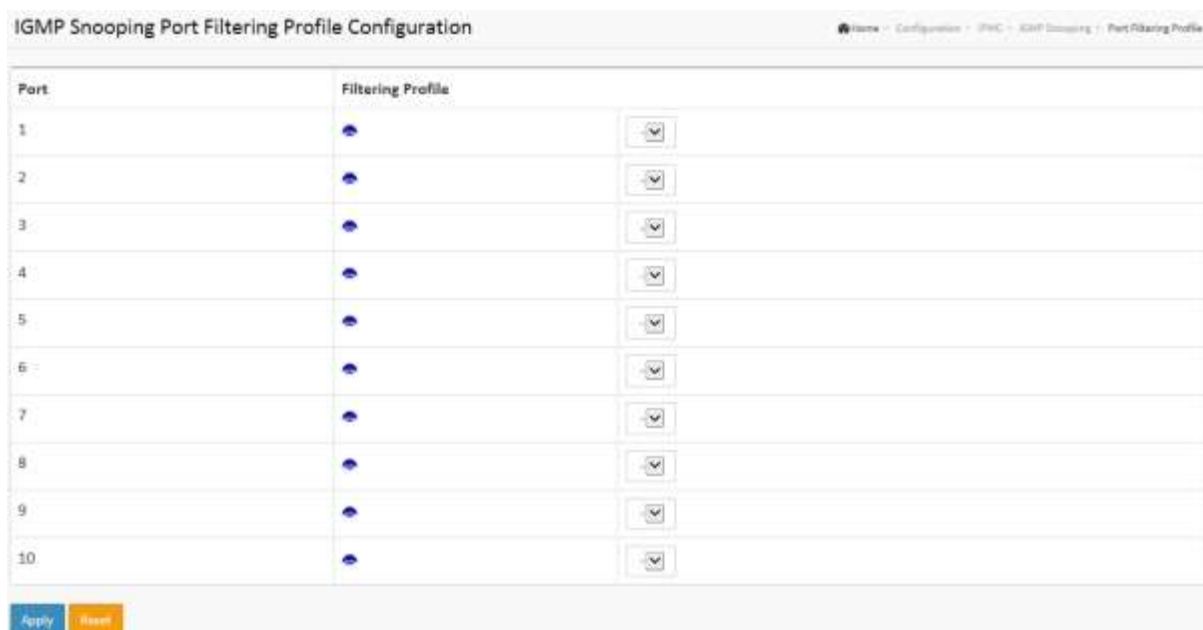
Figure 2-11.1.3: The IGMP Snooping Port Group Filtering Profile.
